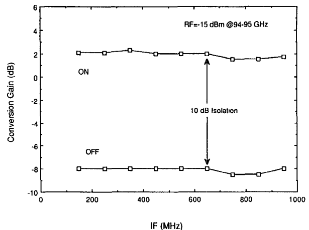
Fig.4 The receiver frequency response with switch on and off by measuring from one IF port of IRM and terminating another IF port with a 50-Ω resistor.
